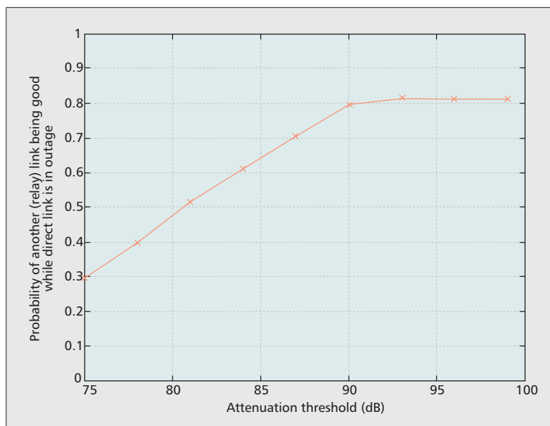
Figure 6. Empirical probability of there being another good (relay) link while the direct link is in outage for a subject sleeping and the hub is situated at the front of the left hip [10].
