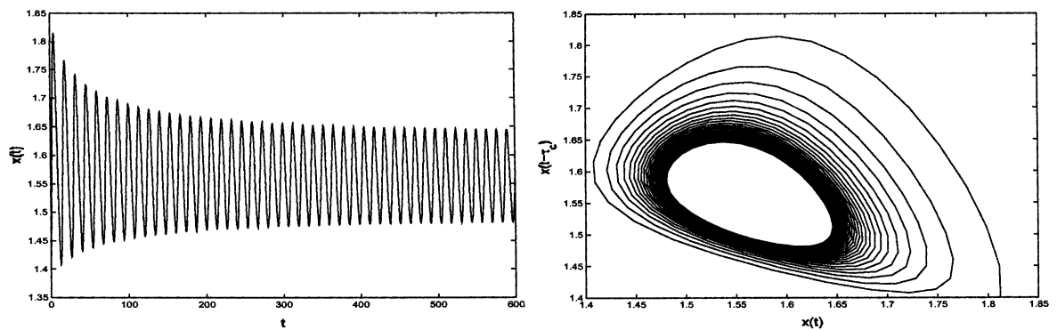
Fig. 7. Solutions of (4) are displayed when n = 8 . Periods of the oscillations are close to 13 days.
