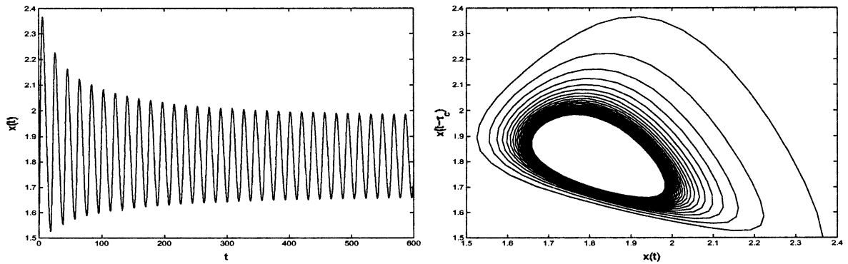
Fig. 5. Solutions of (4) are displayed when n = 6 . Periods of the oscillations are close to 18 days.
