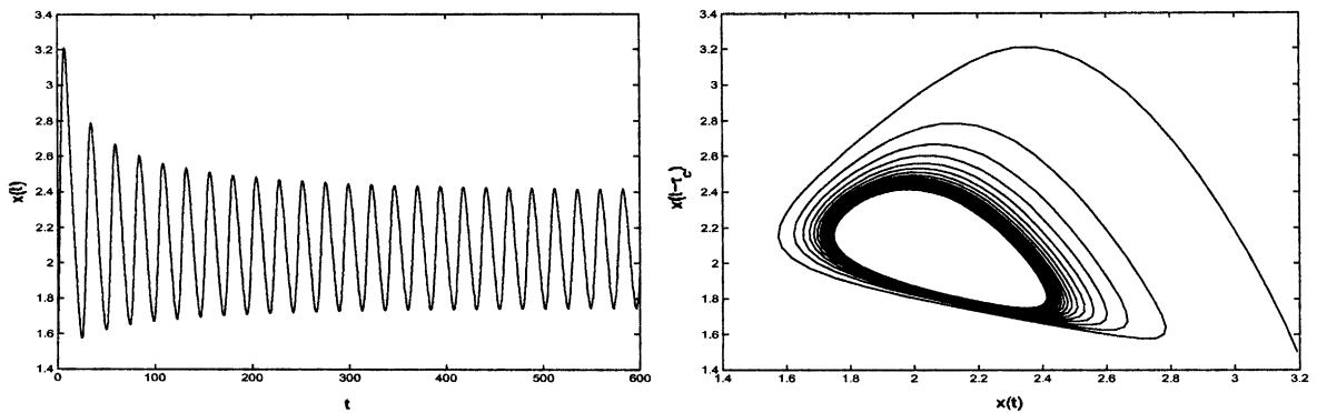
Fig. 4. Solutions of (4) are displayed when n = 5 . Periods of the oscillations are close to 23 days.
