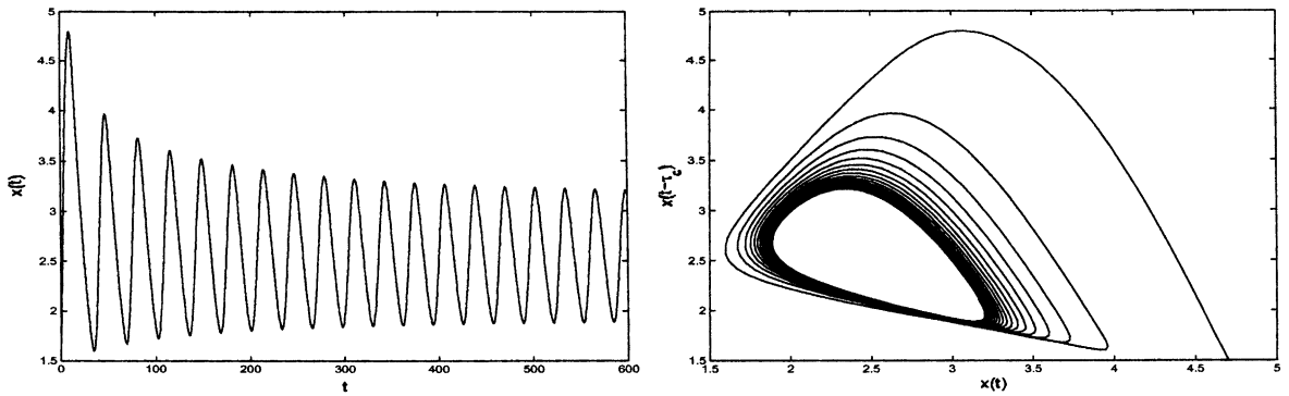
Fig. 3. Solutions of (4) are displayed when n = 4 . Periods of the oscillations are close to 30 days.
