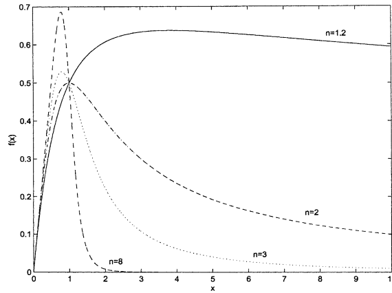
Fig. 1. Graph of the function f given by (5) for different values of n .
