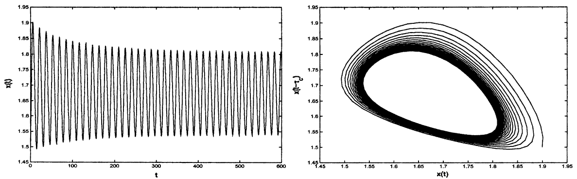
Fig. 6. Solutions of (4) are displayed when n = 7 . Periods of the oscillations are close to 15 days.
