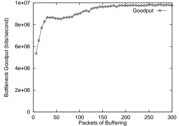
Figure 9: Buffers vs. Goodput for 30 TCPs
