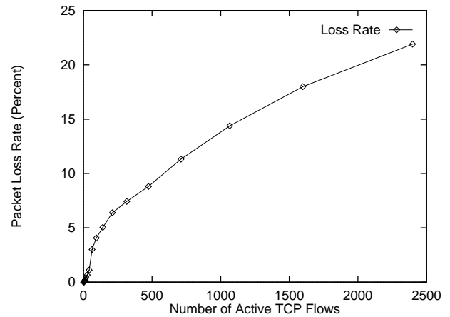
Figure 7: Number of Flows vs. Loss Rate
