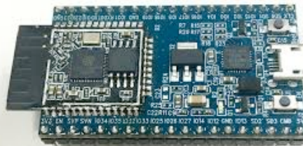
Expressif ESP32
