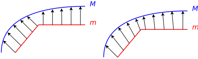
Figure 2: Throwing rays with interpolated normal (right) rather than the triangle normal as directions avoids sampling discontinuities.
